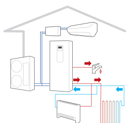
EHS TDM PLUS + ClimateHub
